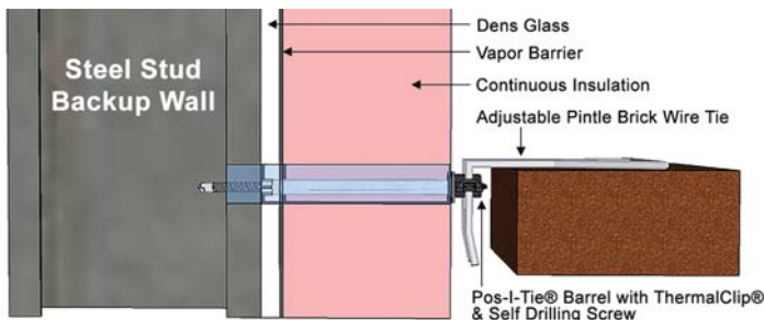
The ThermalClip® is secured when both sides are snapped into place.
