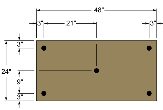
24 in. x 48 in. Panel with 5 Fasteners
