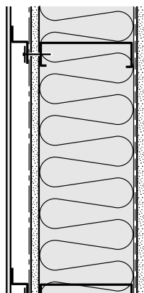
Stud Cavity Insulated
