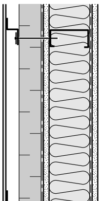
Split Insulated
