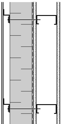
Exterior Insulated
