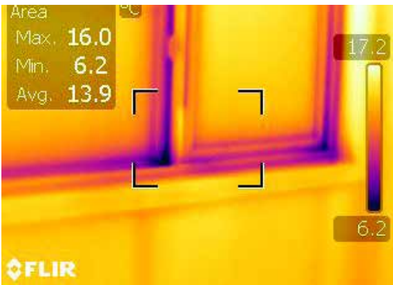
Figure 6: Thermal penetration observed around window frame on main level. Source: SAIT
