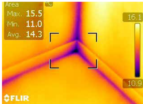
Figure 7: Thermal penetration observed between wall and floor assembly connections on main level. Source: SAIT
