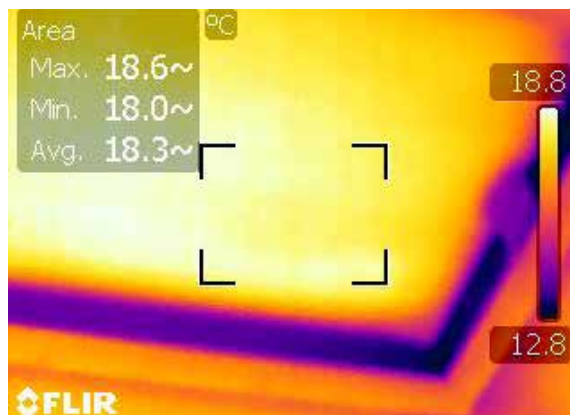
Figure 9: Thermal leakage observed around the attic hatch. Source: SAIT
