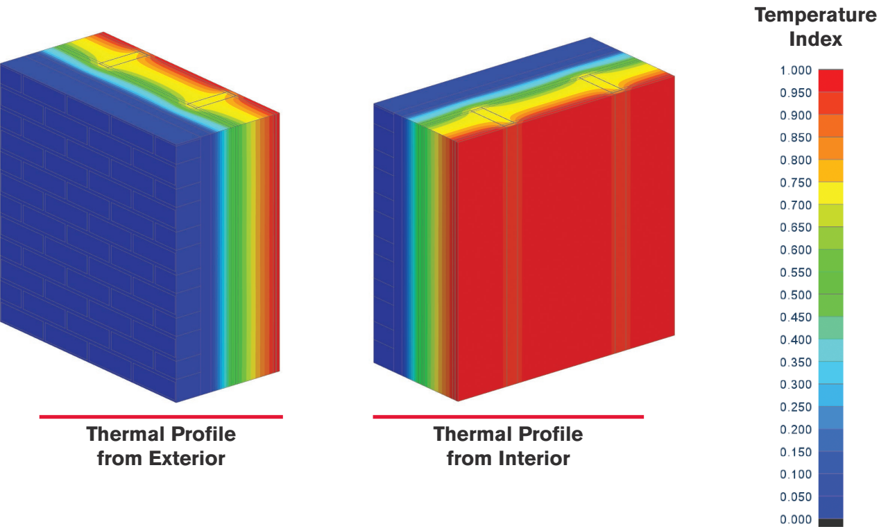
(3" Exterior Insulation and R-20 Batt Insulation scenario shown)
