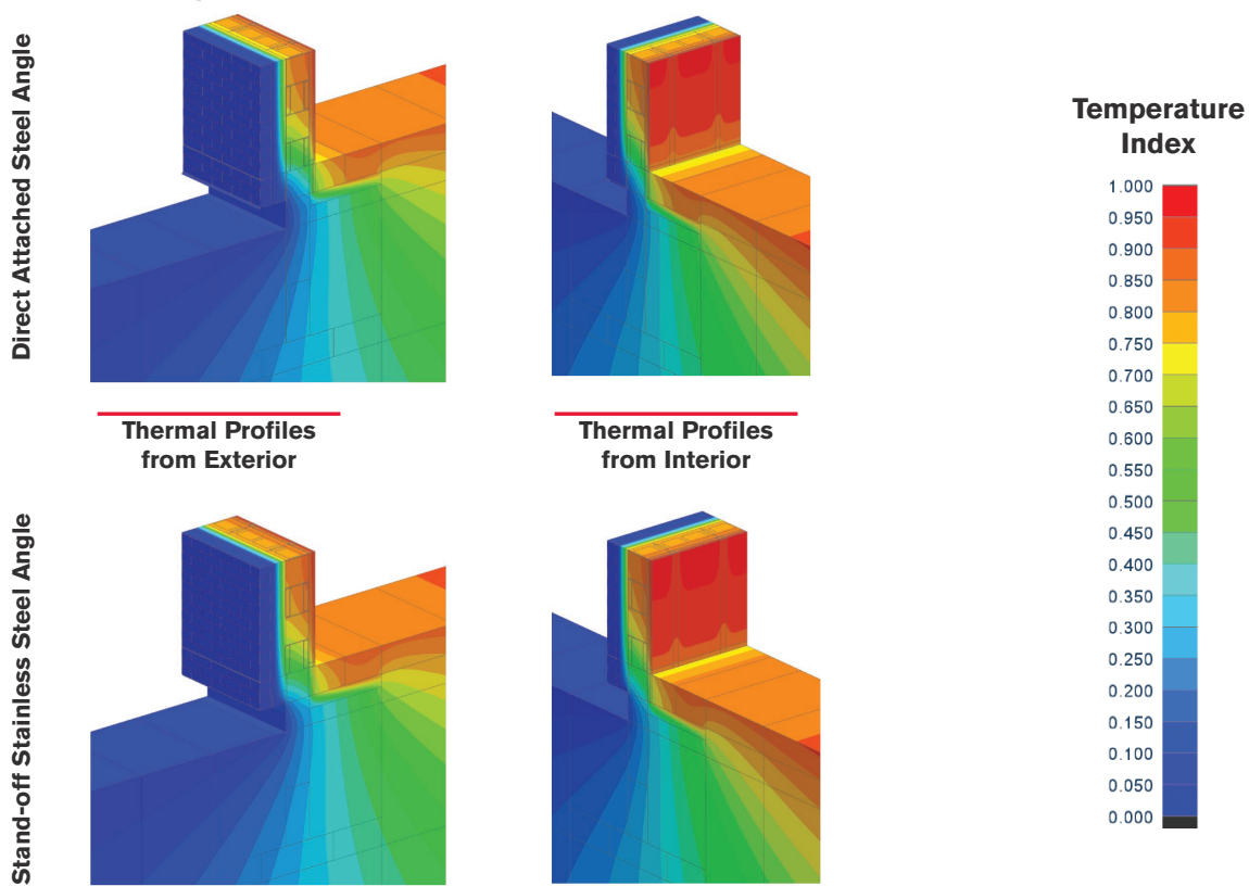
(4" Exterior Insulation scenario shown)
