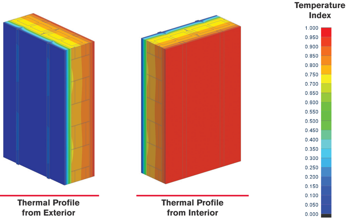
(3" Exterior Insulation scenario shown)
