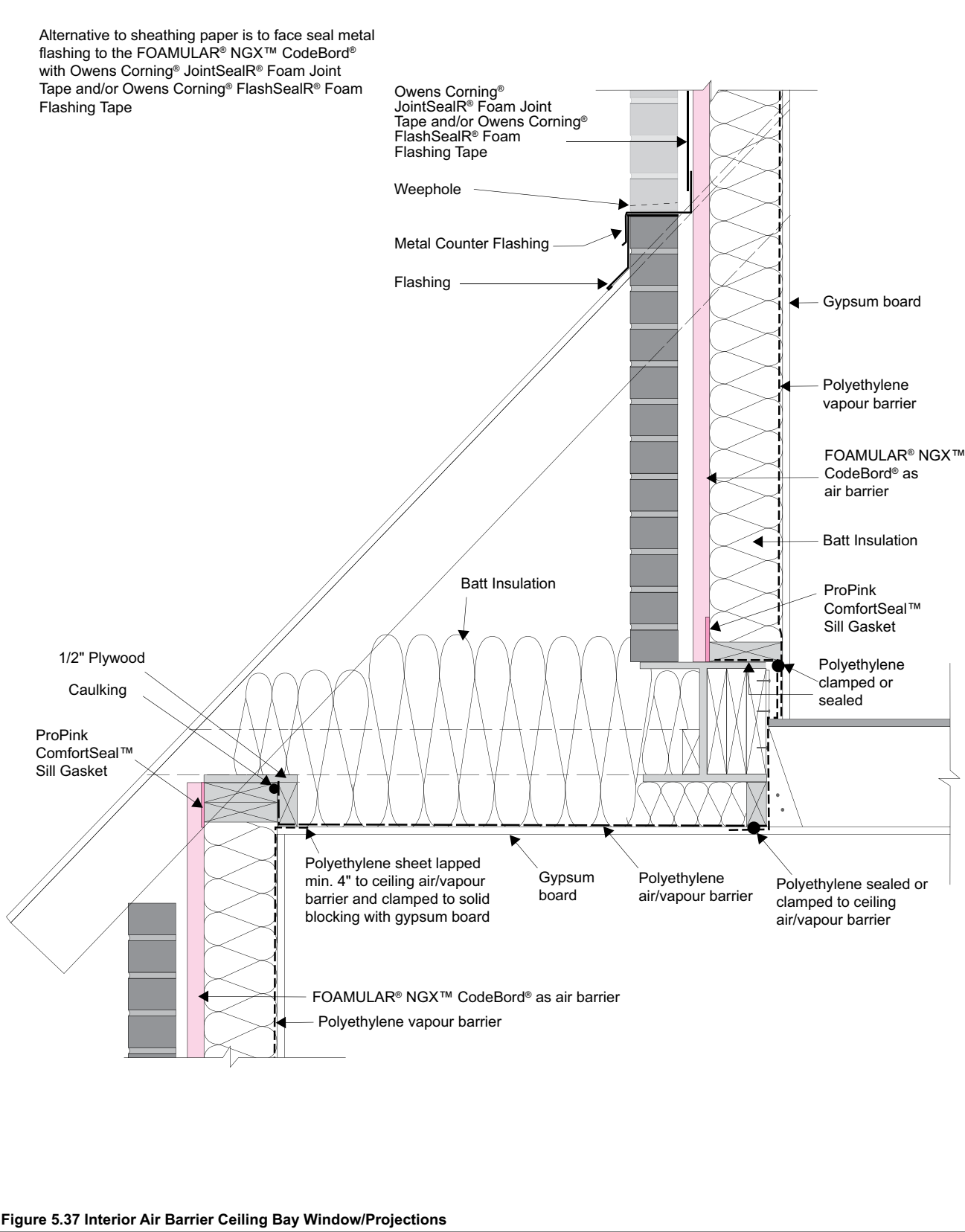
Figure 5.37 Interior Air Barrier Ceiling Bay Window/Projections
