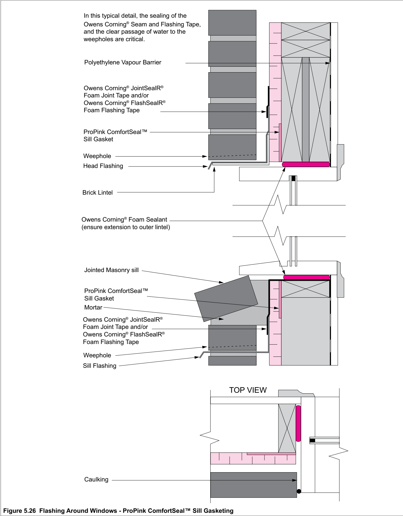
Figure 5.26 Flashing Around Windows - ProPink ComfortSeal™ Sill Gasketing
