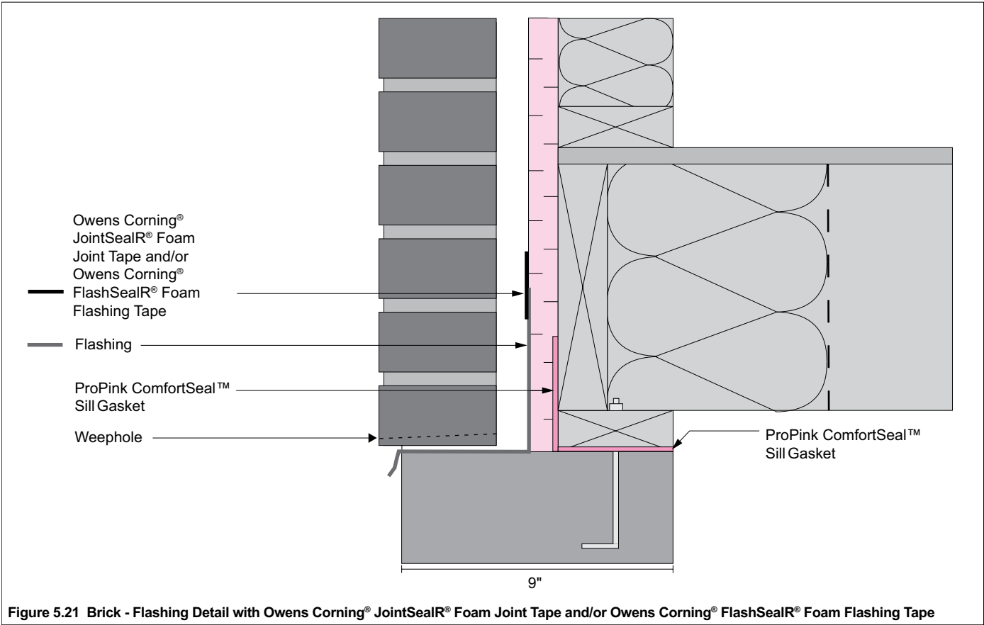
Figure 5.21 Brick - Flashing Detail with Owens Corning® JointSealR® Foam Joint Tape and/or Owens Corning® FlashSealR® Foam Flashing Tape
