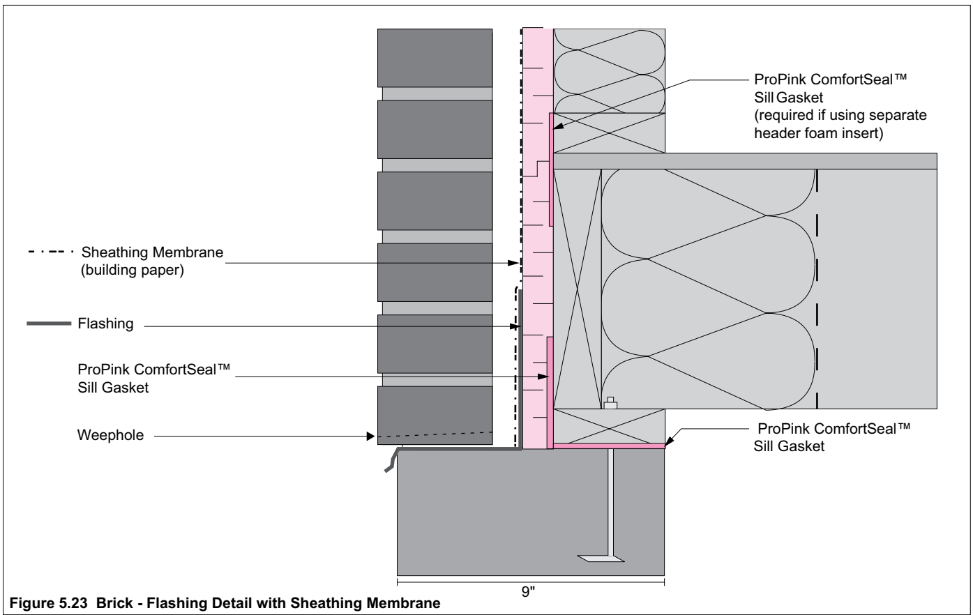
Figure 5.23 Brick - Flashing Detail with Sheathing Membrane
