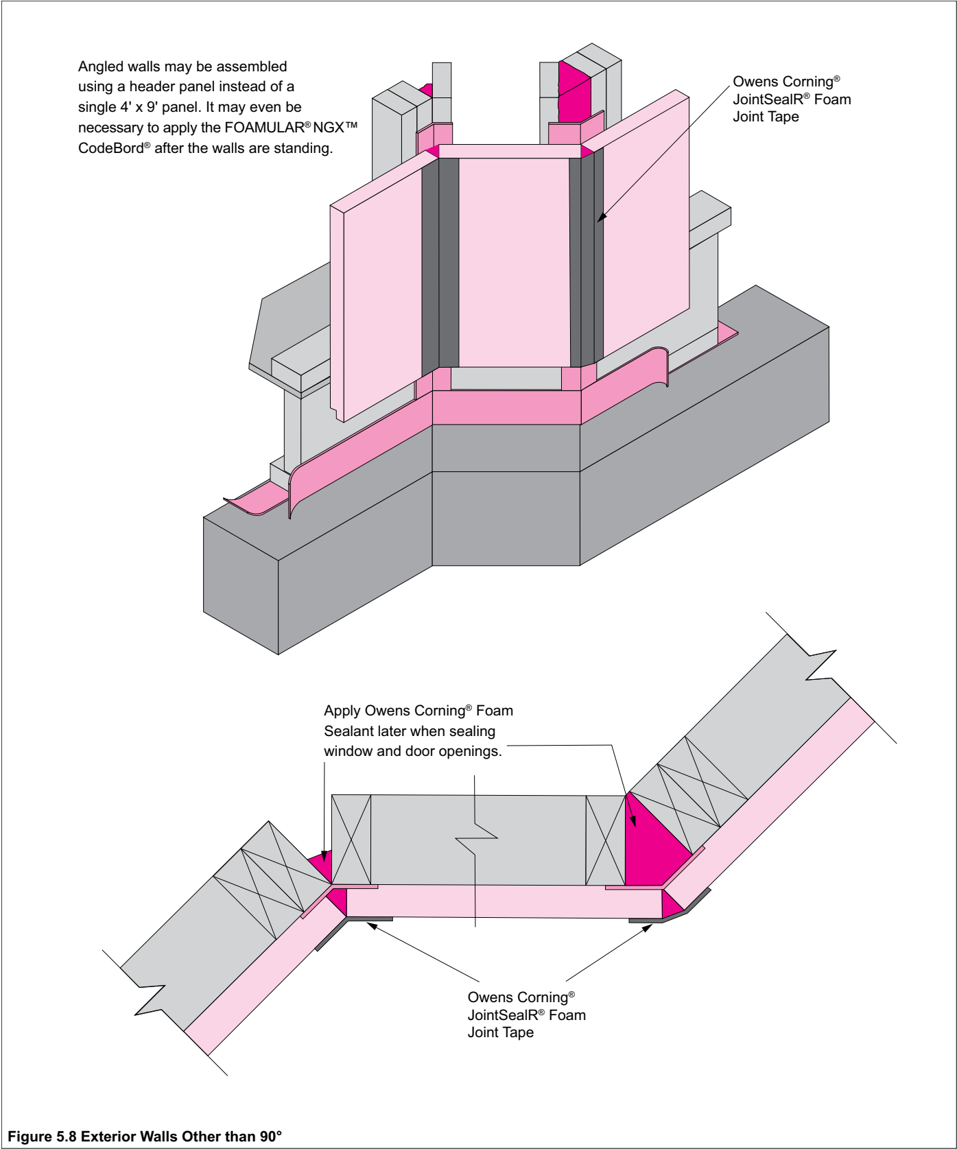
Figure 5.8 Exterior Walls Other than 90°
