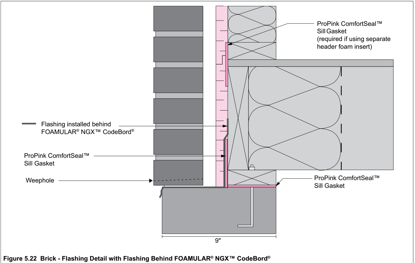
Figure 5.22 Brick - Flashing Detail with Flashing Behind FOAMULAR® NGX™ CodeBord®
