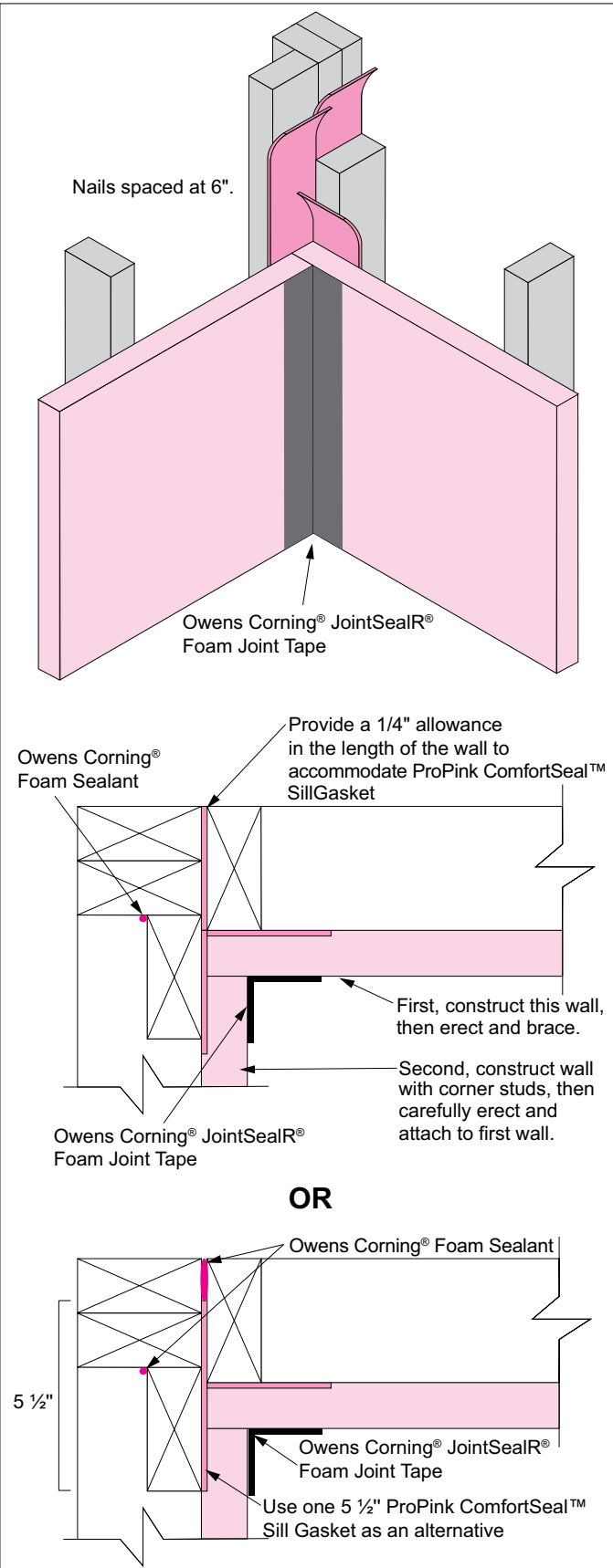
Figure 5.7 Inside Corner of Exterior Wall
